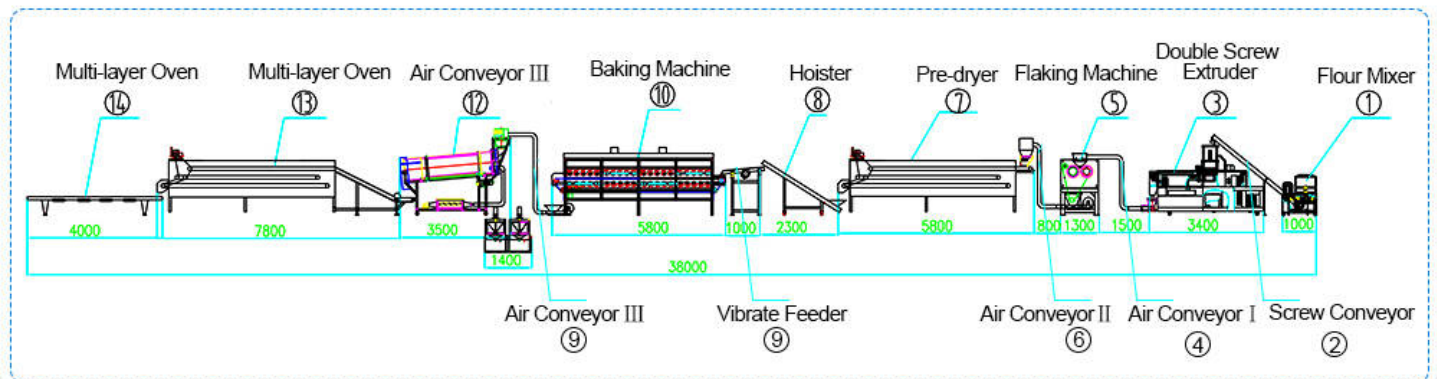
Corn Flakes Making Machine Flow Chart
