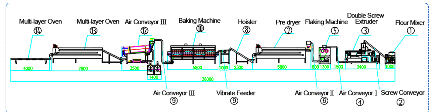
Flow Chart of Corn Flakes Making Machine
