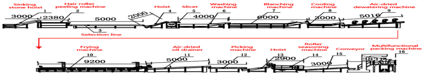
Processing Flow Of Fully Automatic Potato Chips Line
