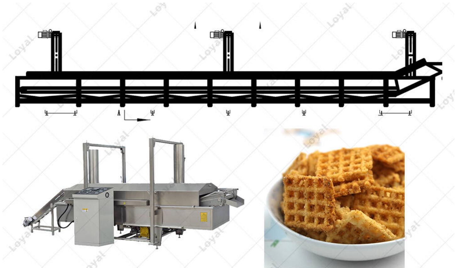
CAD Of Industrial Salad Snack Fryer Production Equipment Technical Parameter Of Industrial Automatic Continuous Salad Snack Fryer Machine Frying Plant
