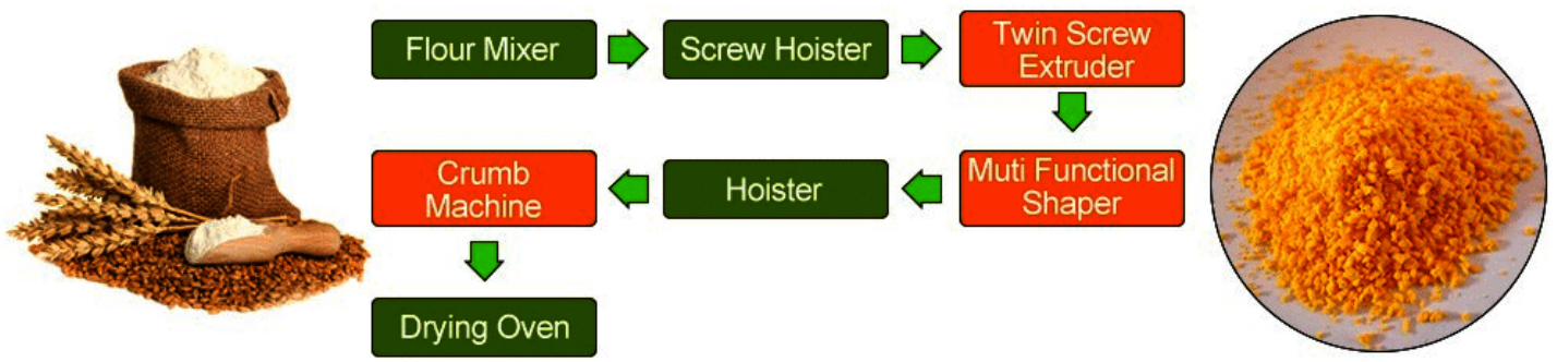
Flow Chart of Bread Crumbs Making Machine
