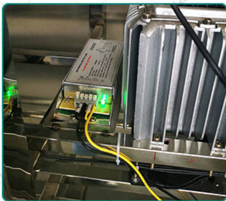
Detail of Tenebrio Mealworm Insect Microwave Drying Sterilization Machine
