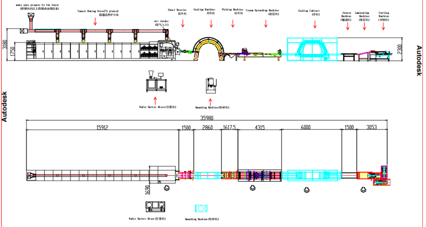
75模平板威化线布置图 75 plates wafer biscuit production line
